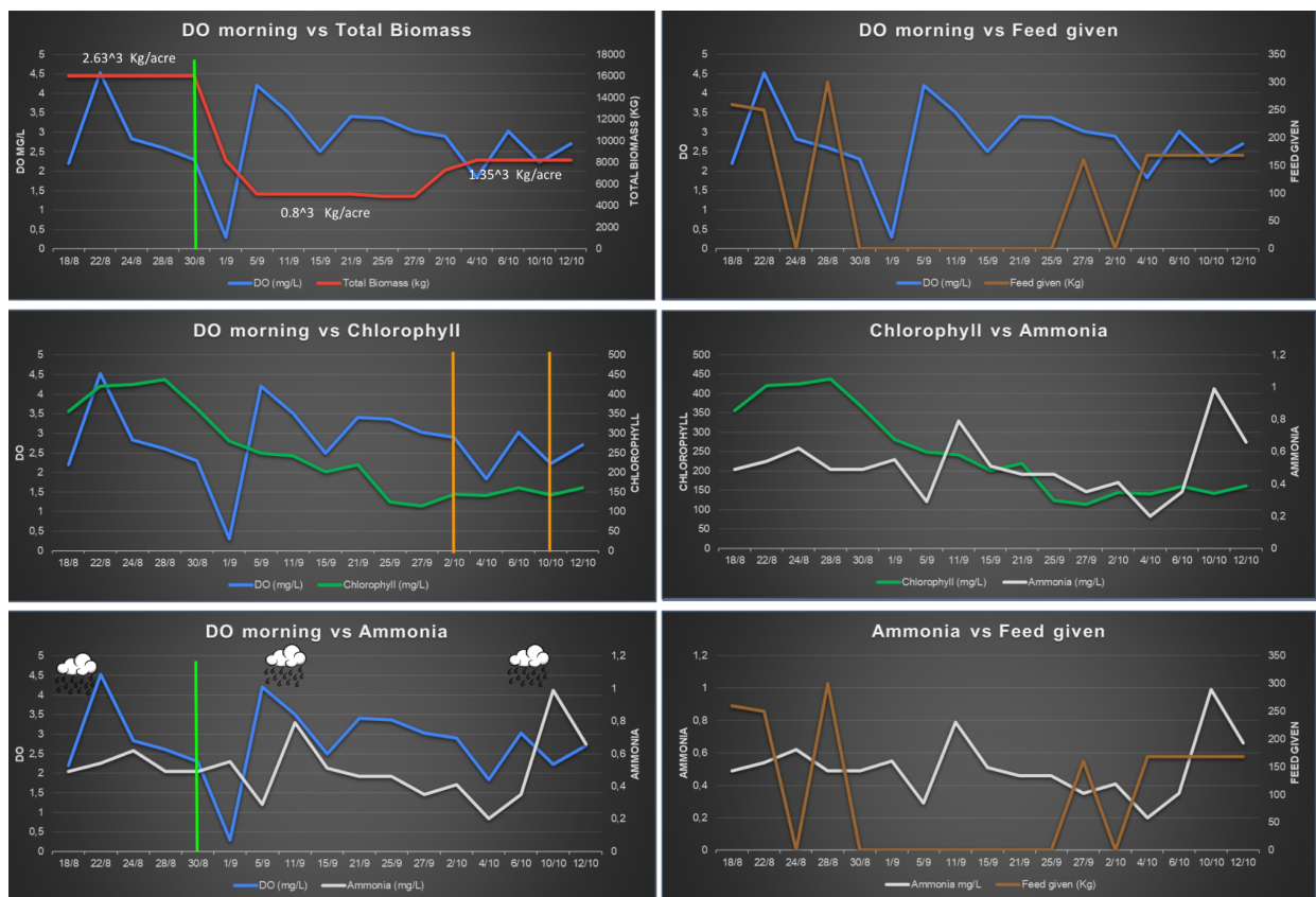
Fig 9: DO measurements at AJU2
