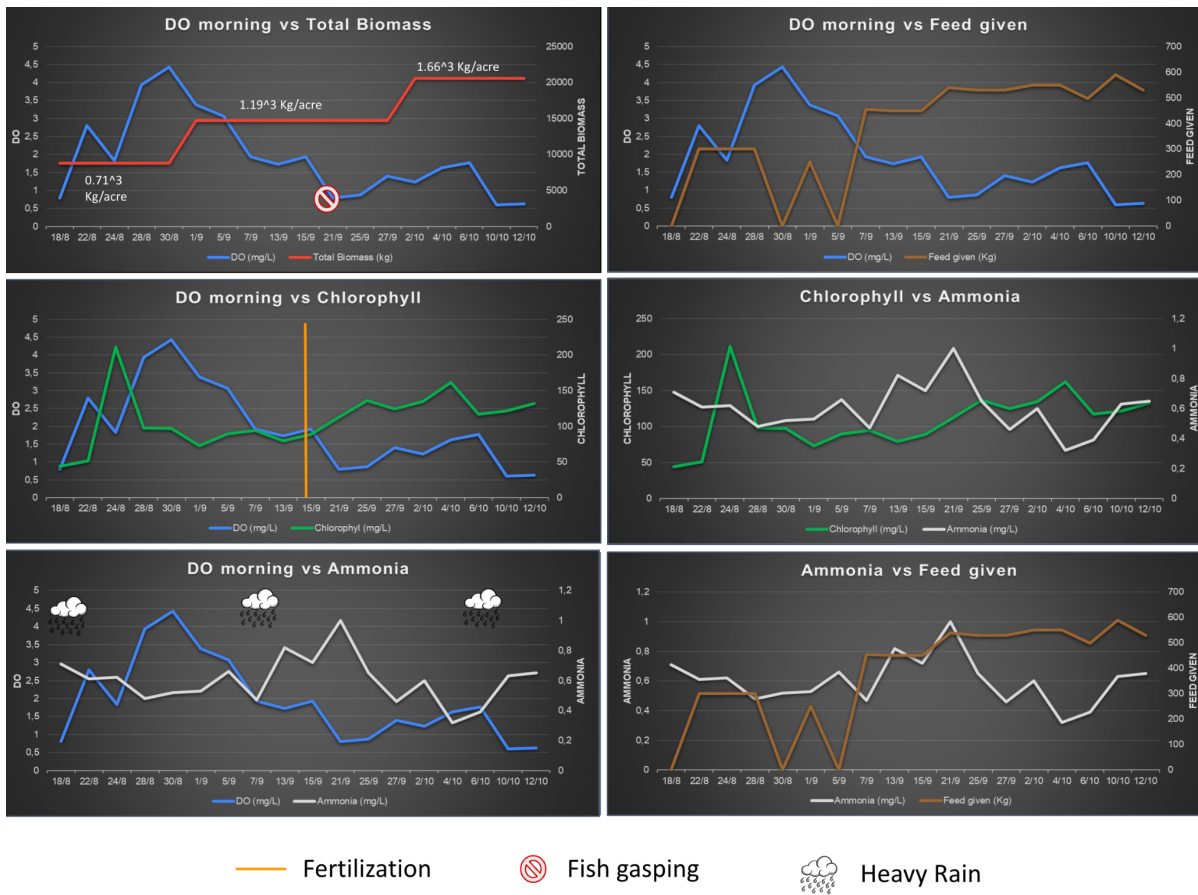
Fig 11: DO measurements at VMS
